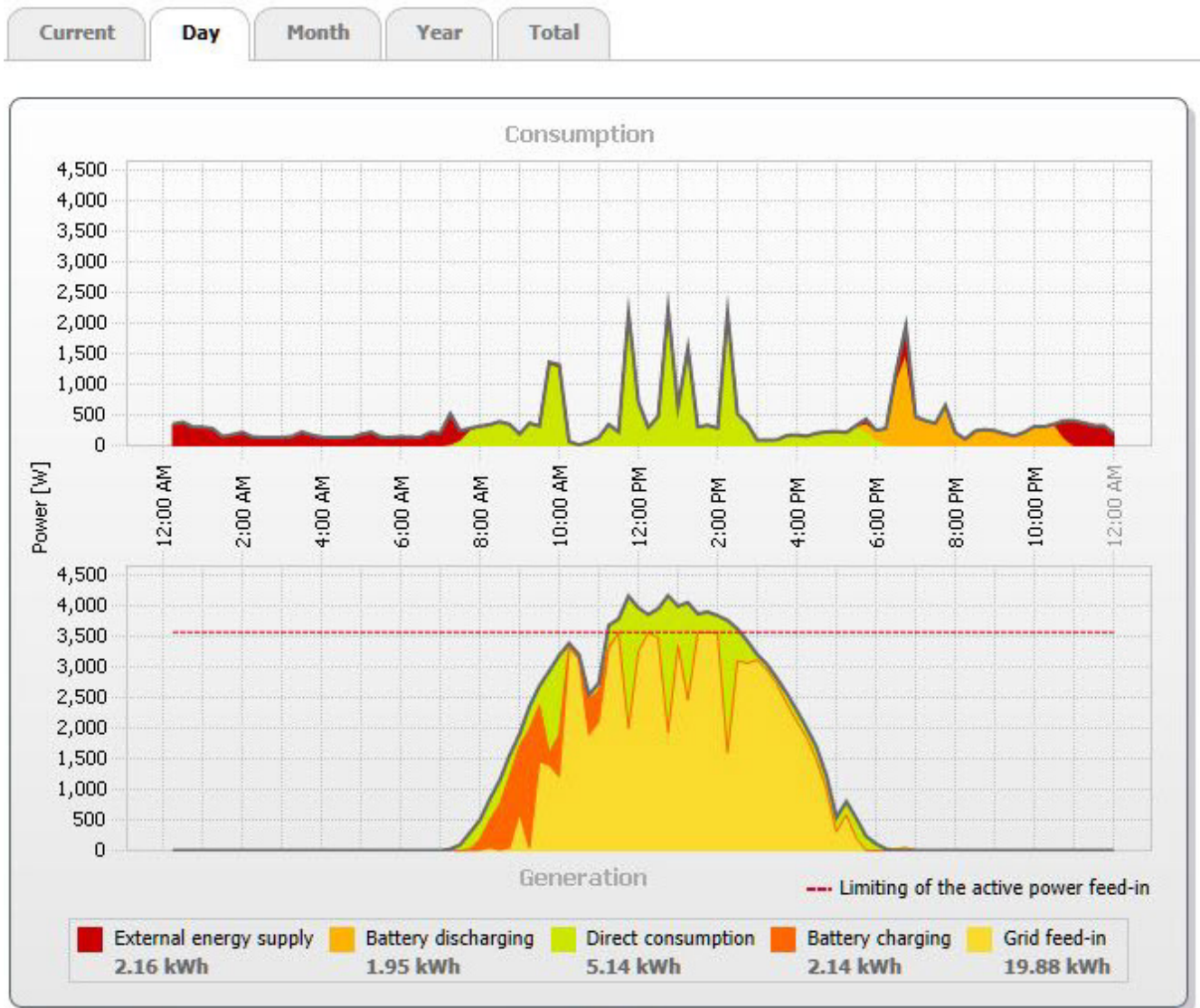
Figure 14: Consideration of PV generation and consumption in Sunny Portal (example 3)
