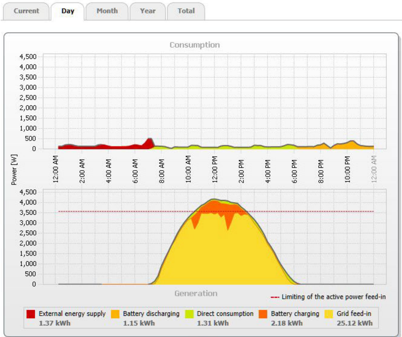
Figure 12: Consideration of PV generation and consumption in Sunny Portal (example 1)
