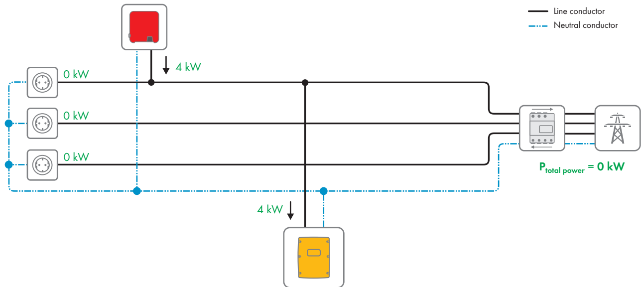
Figure 17: The battery inverter charges the battery.
