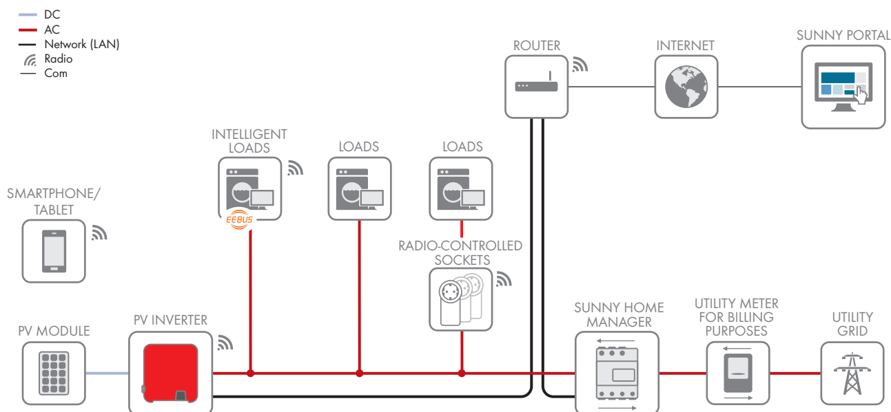
Figure 25: Control of household appliances in the SMA Smart Home
