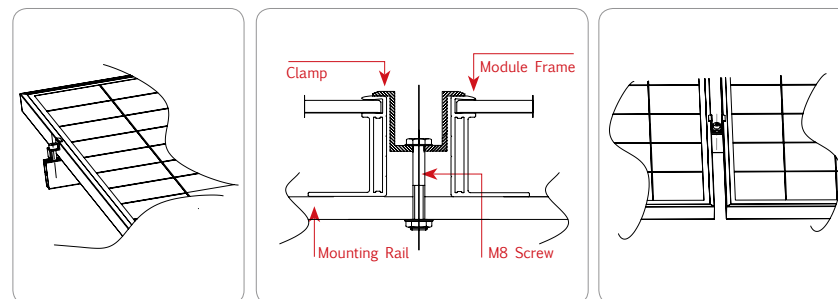
Module installed using Clamp Fitting method (The minimum recommended length for each clamp is 50 mm)
