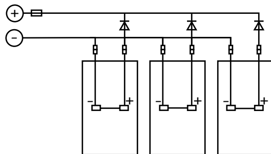
Parallelschakeling
