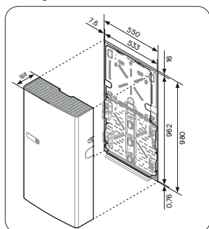
Wandmontage (inbegrepen)
