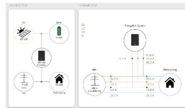
The flow of power and current through your EnergyHub system. The power flow provides an overview of your system. Where the energy is going right now, how much solar electricity you are producing and whether your battery is charging or discharging. The diagram provides an overview of your building per phase, as well as the rating of the building's main fuse.
