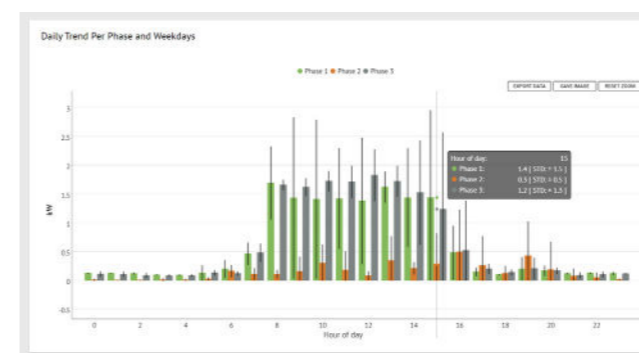
Load profiles provide you with an overview of the loads placed on your grid connection over a selected 24-hour period. This is an important tool for assessing load variation over the course of the day in order to assess your own use of solar electricity. It also shows the disparity between weekdays and weekends.
