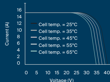
Current-Voltage (440W)
